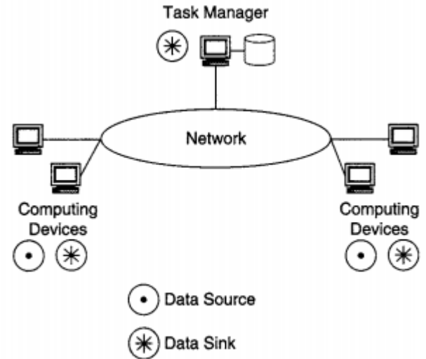
FIGURE 5.15 The Distributed-Computing Architectural Model
